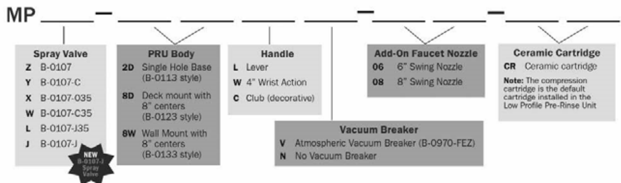
Low Profile Pre-Rinse Unit Configurator – Build Your Own Low Profile Pre-Rinse!
