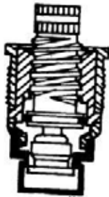
American Standard Aquaseal stem.
