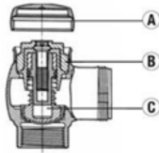
H-700 Stop, chrome plated: Screwdriver Angle Stop with H-1010-A Vandal Resistant Cap
