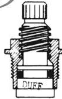
Central Lav Stem
