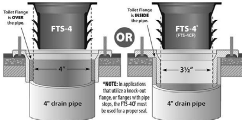
The NEW FTS-4 Wax Free Toilet Seal
