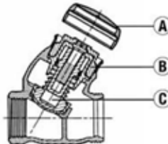
H-750 Stop, chrome plated: Screwdriver Straight Stop with H-1010-A Vandal Resistant Cap
