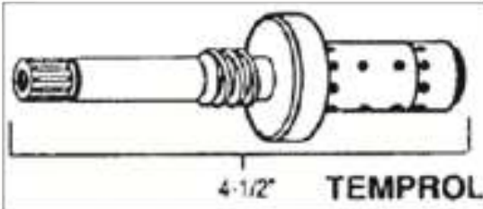
4-1/2" TEMPROL Temprol spindle assembly TA-10
