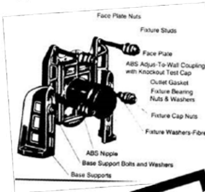
Chair Hanger, Wall Hung Toilet Support
