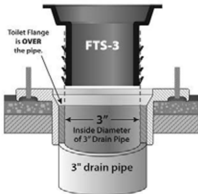
The FTS-3 Wax Free Toilet Seal
