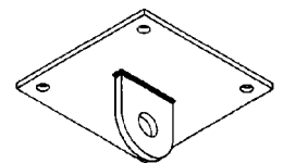
STRUCTURAL WELD- ING LUG 1/2 TO 3 3/4"ROD
